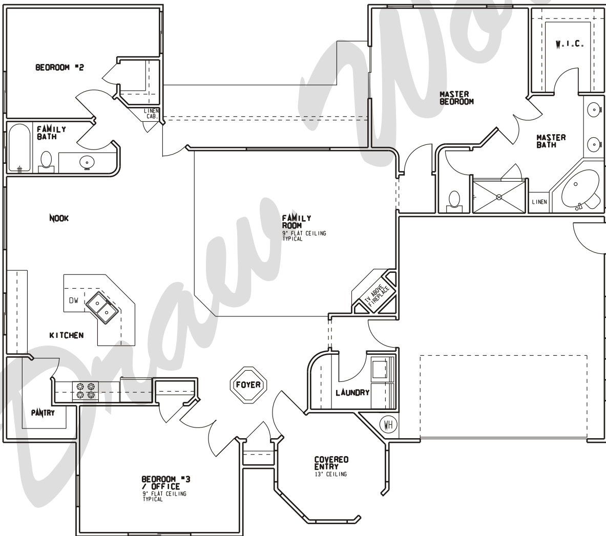
FLOOR PLAN
